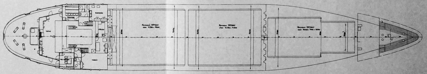
PONT PRINCIPAL
